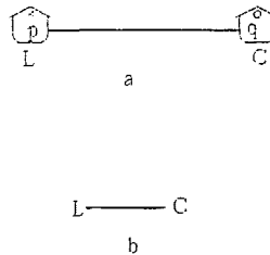
figure 2 Harmonic oscillator
